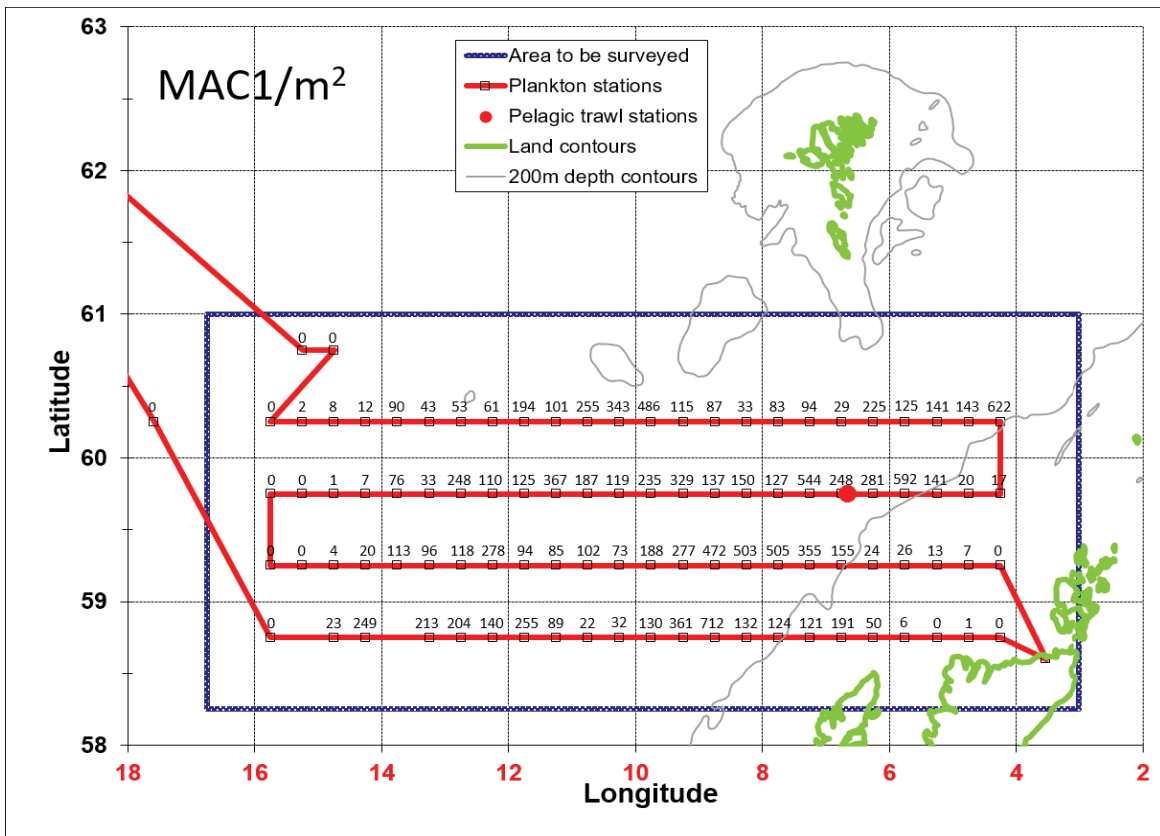
Figure 3. Number of stage 1 mackerel eggs during the research cruise B8-2016, 2 - 16 May 2016 (period 5).
