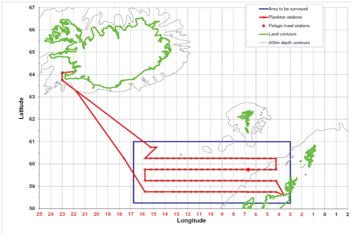
Figure1. The route and plankton- and CTD stations worked of RV. Bjarni Sæmudsson during the research cruise B8-2016, 2 – 10 May 2013 (period 5).
