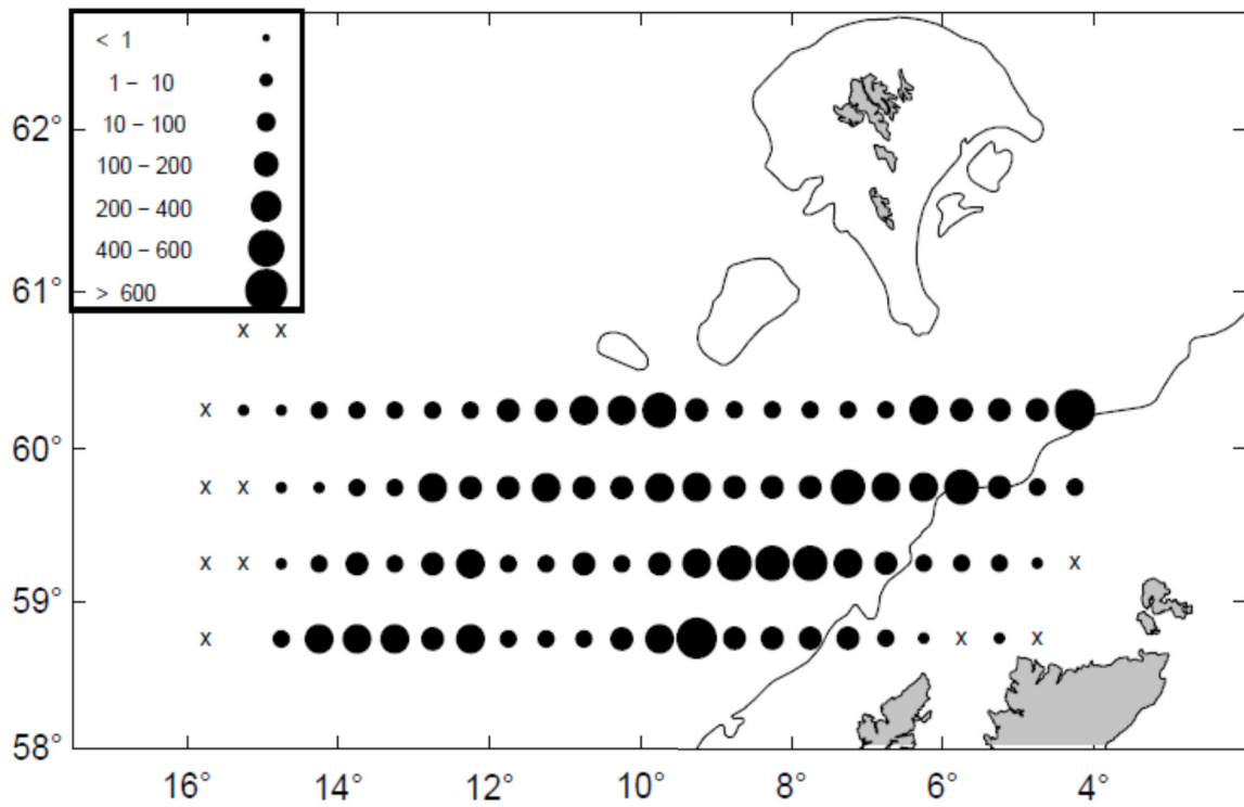
Figure 4. Number of stage 1 mackerel eggs per m 2 during the research cruise B8-2016, 2 - 16 May 2016 (period 5).
