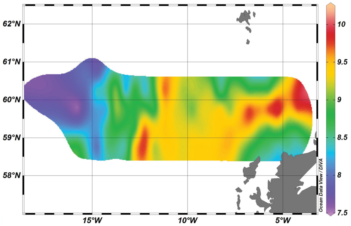
Figure 5. Temperature at the surface (5m) during the research cruise B8 – 2016, 2 – 16 May 2016 (period 5).
