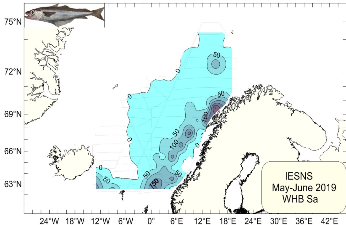
Figure 18. Distribution of blue whiting as measured during the IESNS survey in May 2019 in terms of NASC values ( \text{m}^2/\text{nm}^2 ) (a) averaged for every 1 nautical mile and (b) represented by a contour plot. The stratification of the survey area is shown on the upper map.
