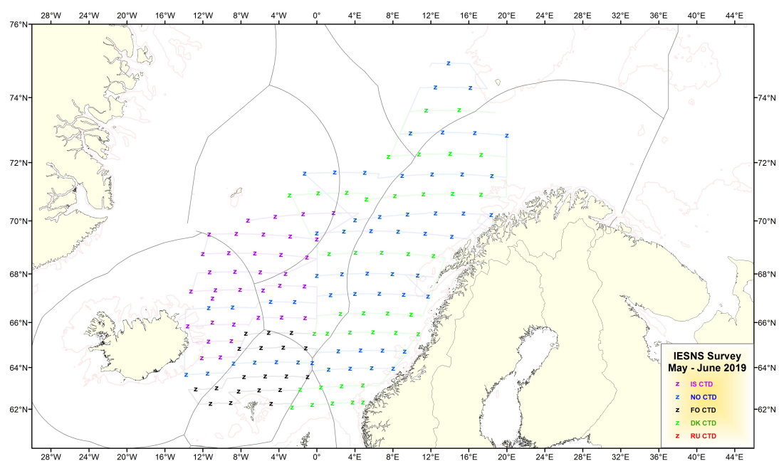
Figure 3a. IESNS survey in May 2019: location of hydrographic stations.
