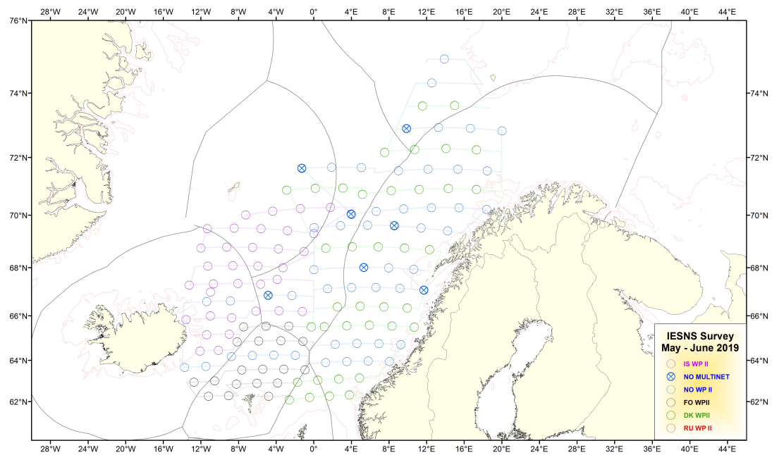
Figure 3c. IESNS survey in May 2019: location of plankton stations
