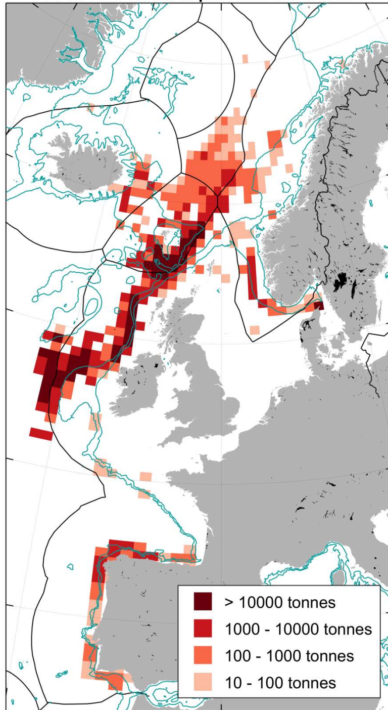
Figure 2.2.1. Blue whiting landings (ICES estimates) in 2017 by ICES rectangle. The 200 m and 1000 m depth contours are indicated in blue. The catches on the map constitute 98.8 % of the total landings.
