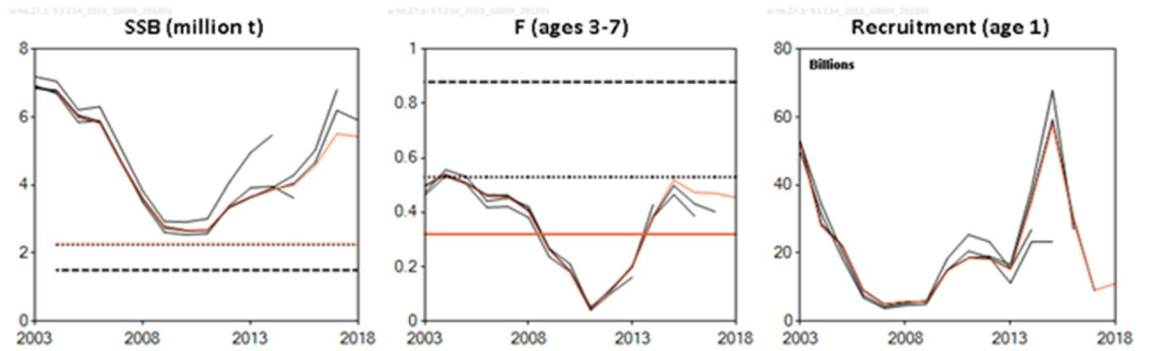
Figure 2.9.1. Blue whiting. Comparison of the 2010 - 2018 assessments.
