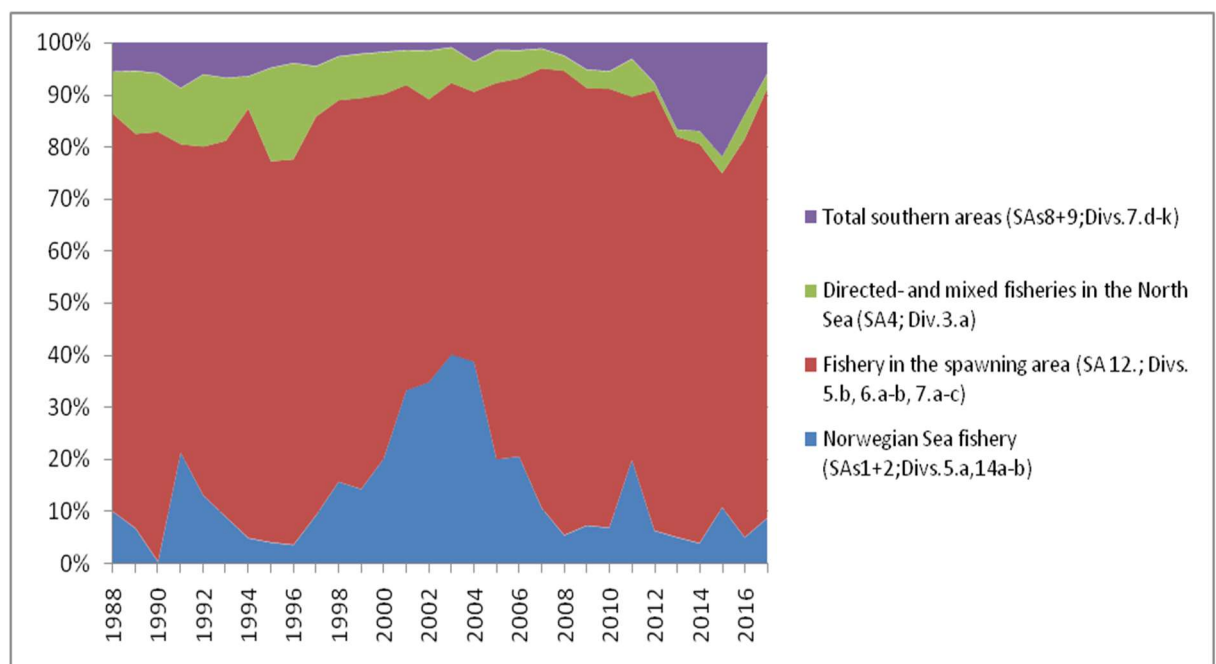
Figure 2.3.1.2. Blue whiting. (A) ICES estimated catches (tonnes) of blue whiting by fishery sub-areas from 1988-2017 and (B) the percentage contribution to the overall catch by fishery sub-area over the same period.
