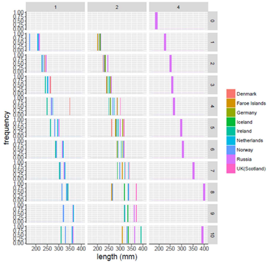
Figure 2.3.1.3.1. Blue whiting. Mean length (mm) by age (0-10 year), by quarter (1,2,4), by country for ICES division area 27.6.a. This data only comprises the 2017 ICES catch-at-age sampled estimates for ICES division area 27.6.a.
