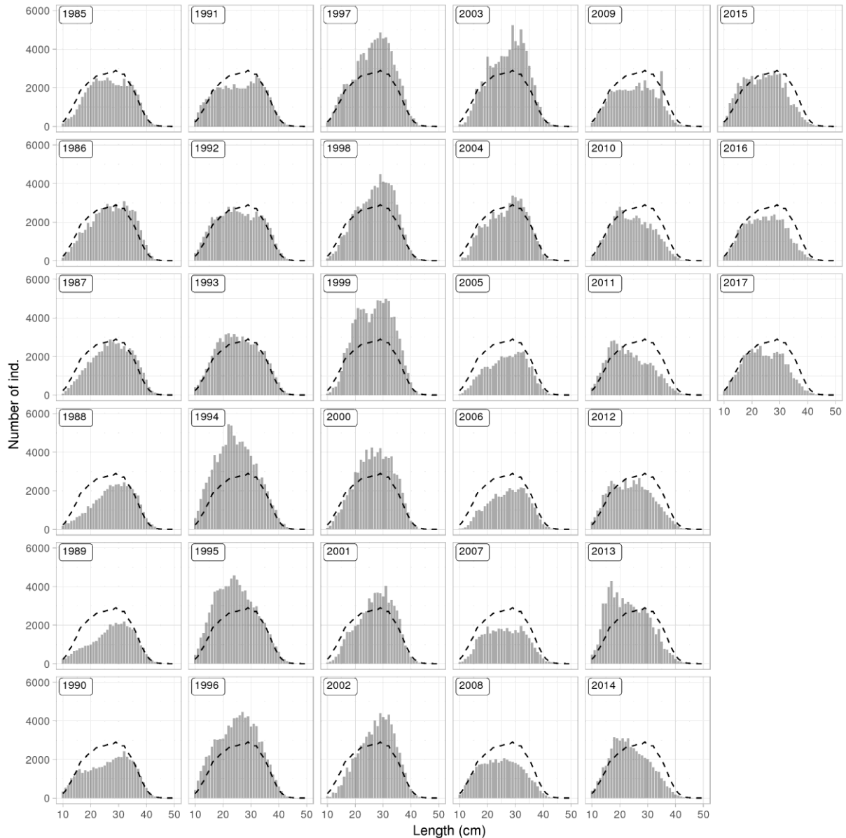
Figure 8. Long rough dab. Length distribution from the spring survey. The dotted line shows mean length distribution for all years combined.
