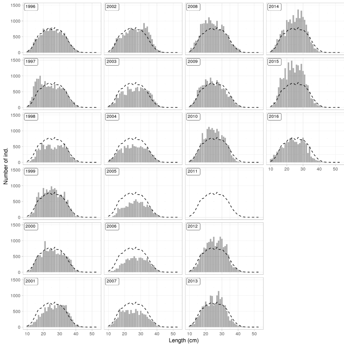
Figure 9. Long rough dab. Length distribution from the autumn survey. The dotted line shows mean length distribution for all years combined.
