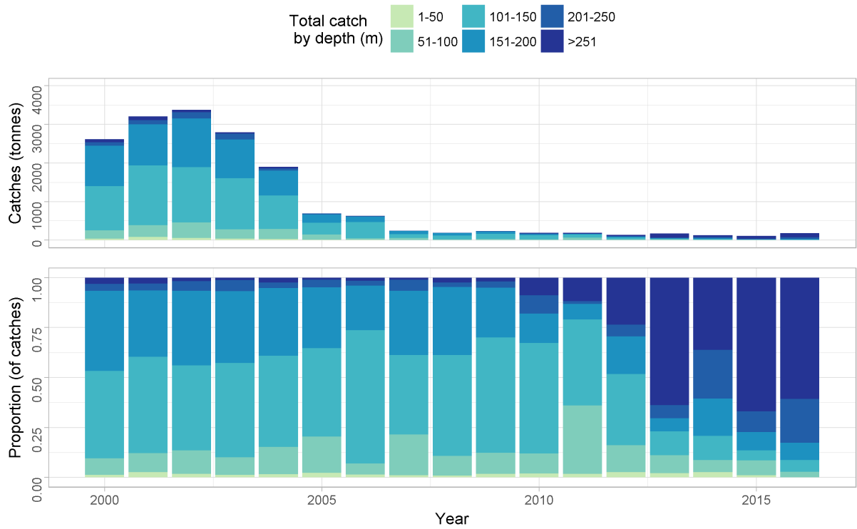
Figure 3. Long rough dab. Depth distribution catches according to logbooks. Mynd 3. Skrápflúra. Afli samkvæmt afladagbókum, skipt eftir dýpi.
