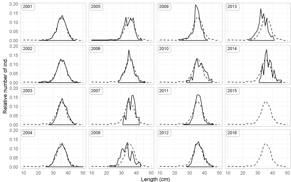
Figure 6. Long rough dab. Length distribution of long rough dab sampled from landed catch. The dotted line represents the mean length distribution for all years.
