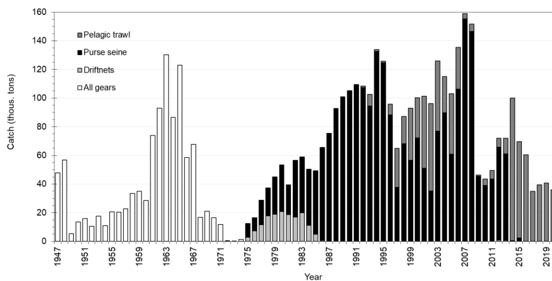
Figure 3. Seasonal total landings (in thousand tonnes) during 1947–2020, referring to the autumns, by different fishing gears from 1975 onwards.
