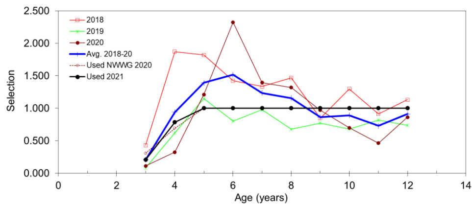
Figure 14. Estimate of selection pattern ( q = F_{\text{age}} / WF_{5-10} ) in the fishery in the stock prognosis for age groups 3 to 12 (+ group) on basis of the F_s in 2018 to 2020, the average over these three years (used for the prognosis), the selection used in 2020 (ICES, 2020), and the selection used in the prognosis 2021.
