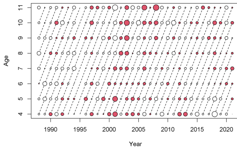
Figure 9. Icelandic summer spawning herring. Residuals of NFT-Adapt run in 2021 from survey observations (moved to 1 January). Filled bubbles are positive (i.e., survey estimates higher than the assessment) and open negative. Max bubble = 1.73.
