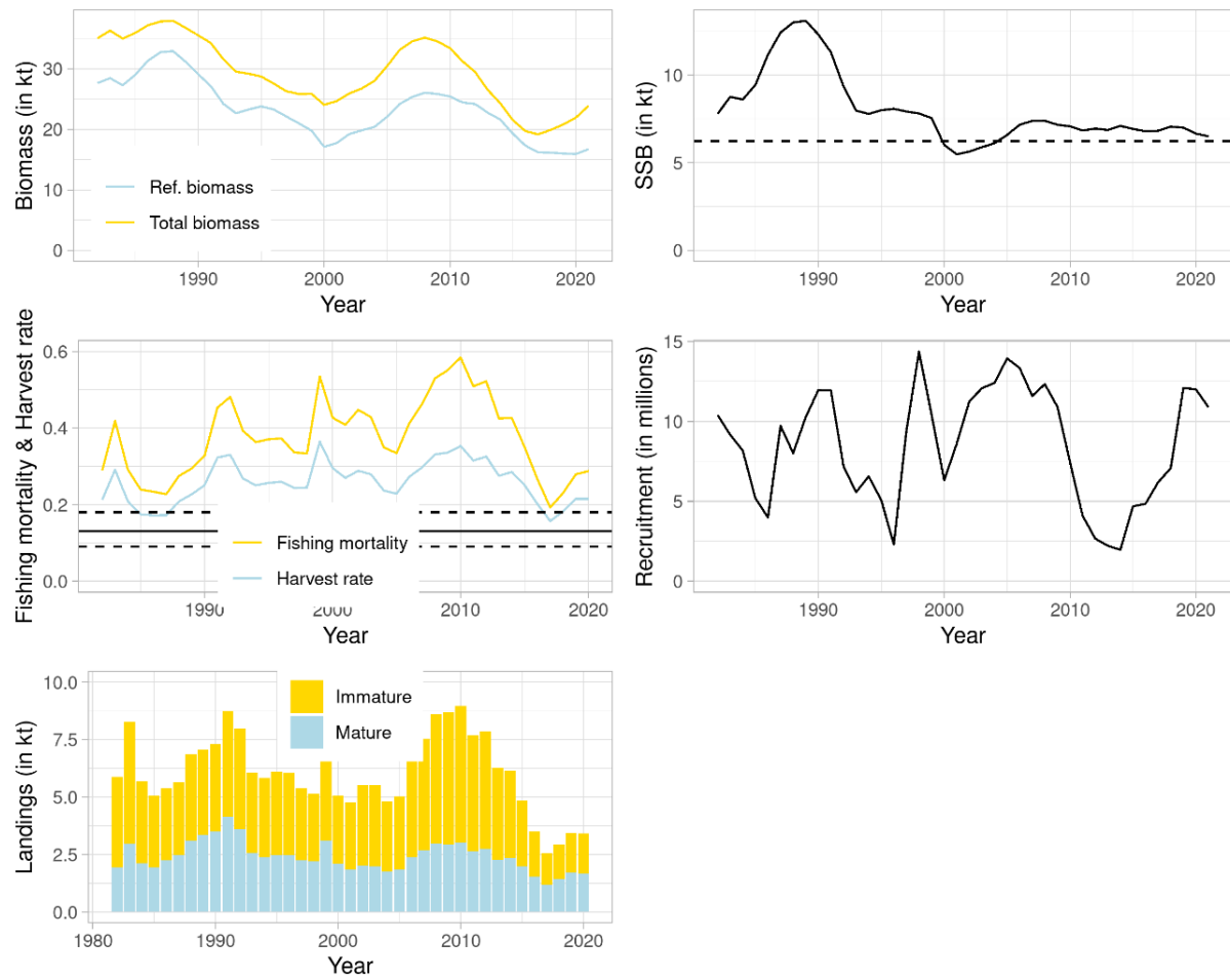
Figure 20. Tusk. Estimated biomass, spawning stock biomass (SSB), fishing mortality for fully selected fish and harvest rate, recruitment, and total catches. The dashed line in the SSB plot represents Bpa. The solid line in the harvest rate plot indicates the target harvest rate used in the harvest control rule, whereas the dashed lines indicate the bounds of the realized harvest rates resulting from the harvest control rule given the uncertainty in the assessment.
