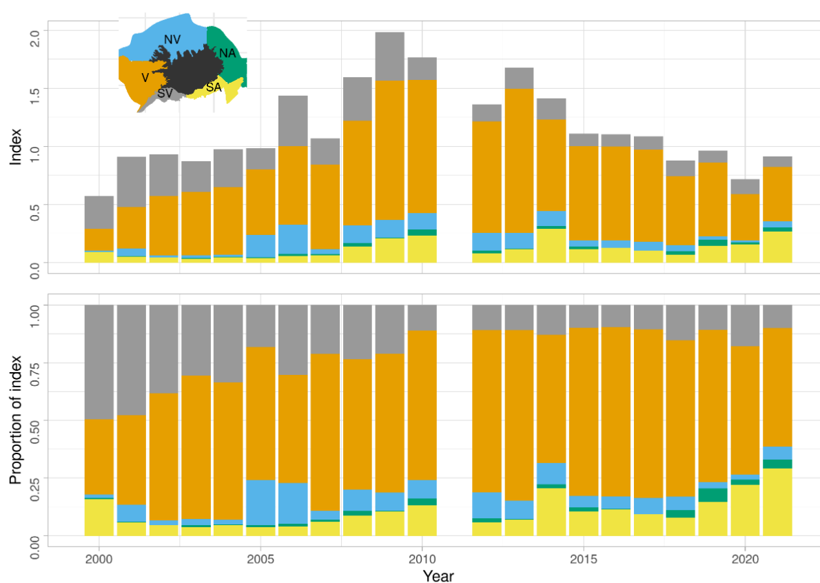
Figure 10. Blue ling. Spatial distribution of biomass index from the Icelandic autumn survey 2000-2021.
