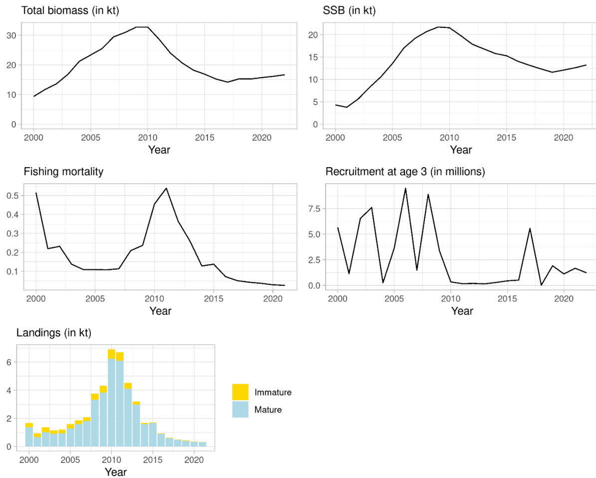
Figure 23. Blue ling. Estimated biomass, spawning stock biomass (SSB), fishing mortality, recruitment, and total catches.
