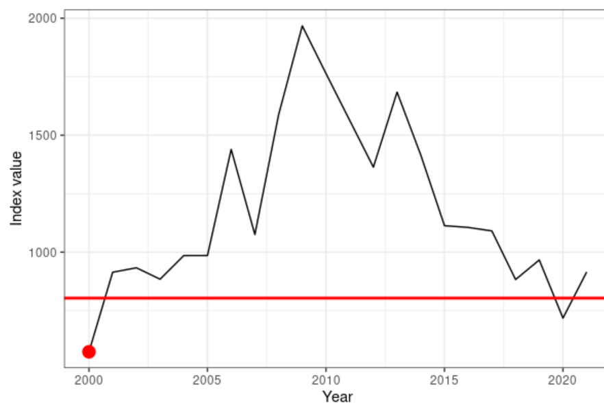
Figure 15. Blue ling. Biomass index values since 2000. The red line is the I_{trigger} and the red dot is the lowest observed value ( I_{loss} ).
