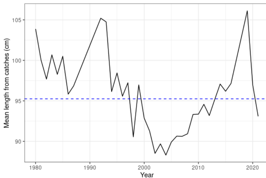
Figure 13. Blue ling. Mean length from catches since 1980. The blue dashed line shows the target reference length.
