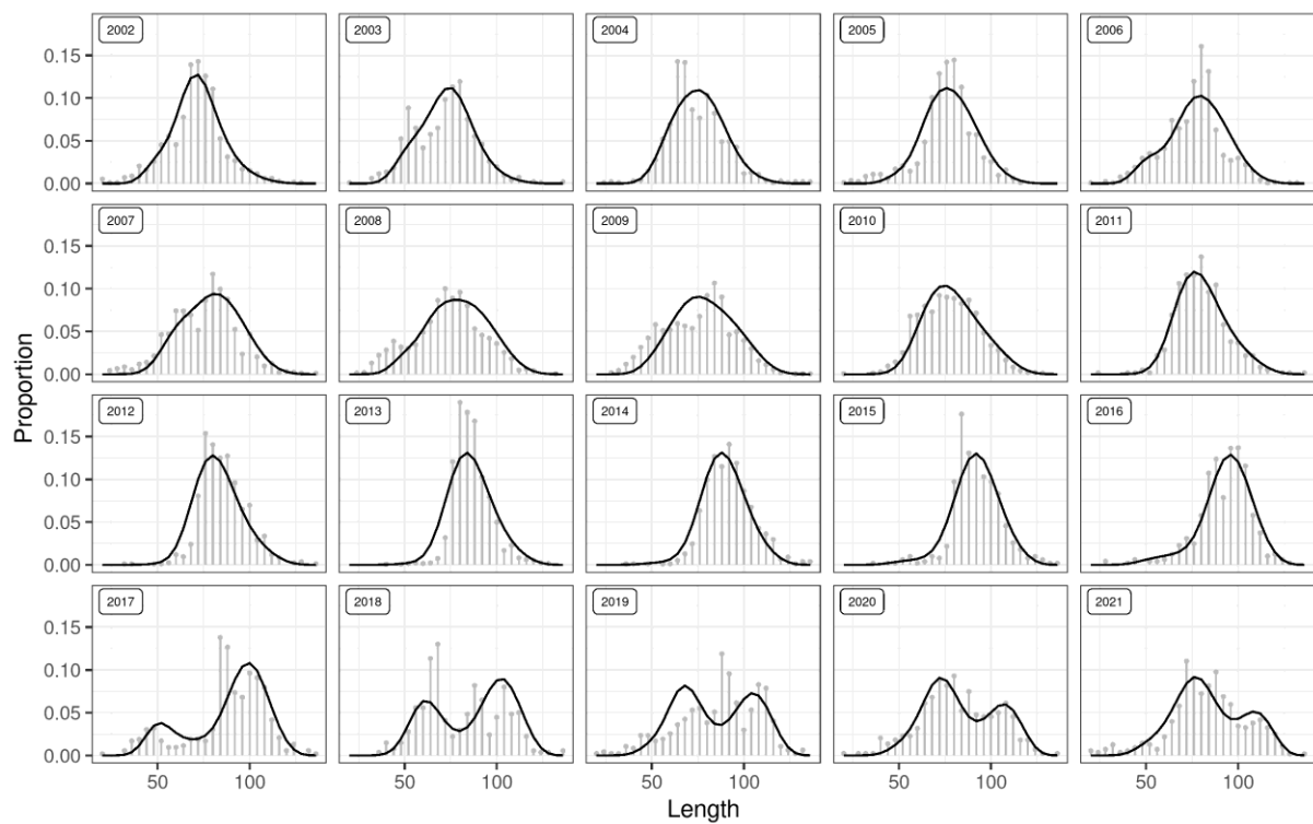
Figure 19. Blue ling. Fitted proportions-at-length from the Gadget model (black lines) compared to observed proportions in the autumn survey (vertical lines and points).
