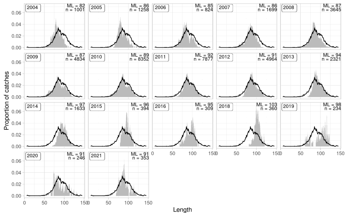
Figure 7. Blue ling. Length distribution of blue ling from trawls and longlines (grey area) of the Icelandic fleet since 2004-2021. Black line is the mean length distribution of the period. No data available in 2017. ML is mean length and n is the number of measurements.
