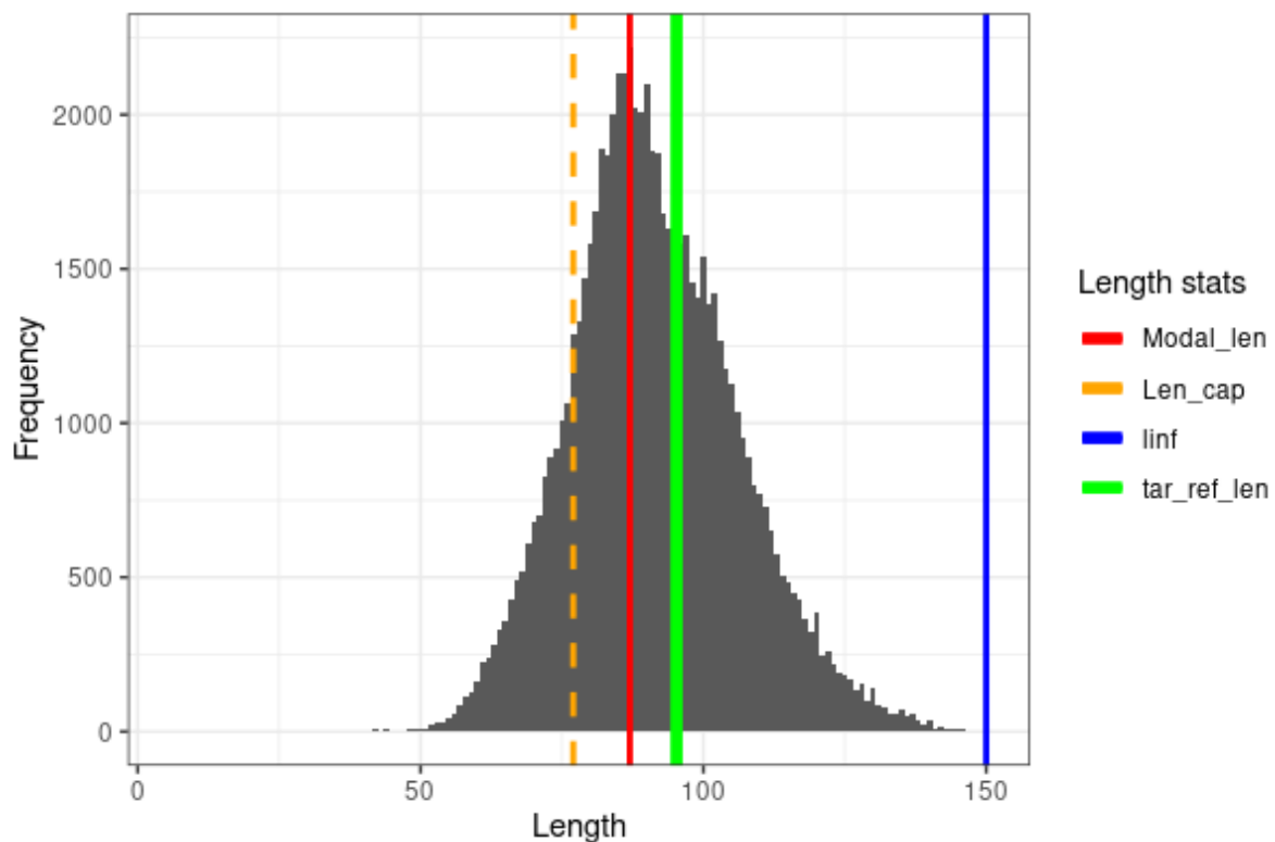
Figure 14. Blue ling. Length frequency distribution from catches. Red line is the length of modal abundance, orange is the length where frequency is half that of the modal value, orange line is the length at first capture, green line is the target reference length, and the blue line is the L_{\infty} .
