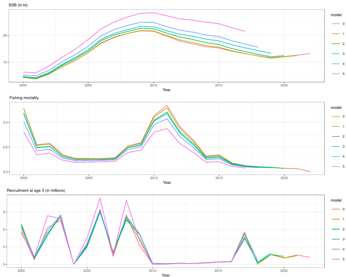
Figure 24. Blue ling. Retrospective plots illustrating stability in model estimates over a 5-year 'peel' in data. Results of spawning stock biomass, fishing mortality F , and recruitment (age 3) are shown.
