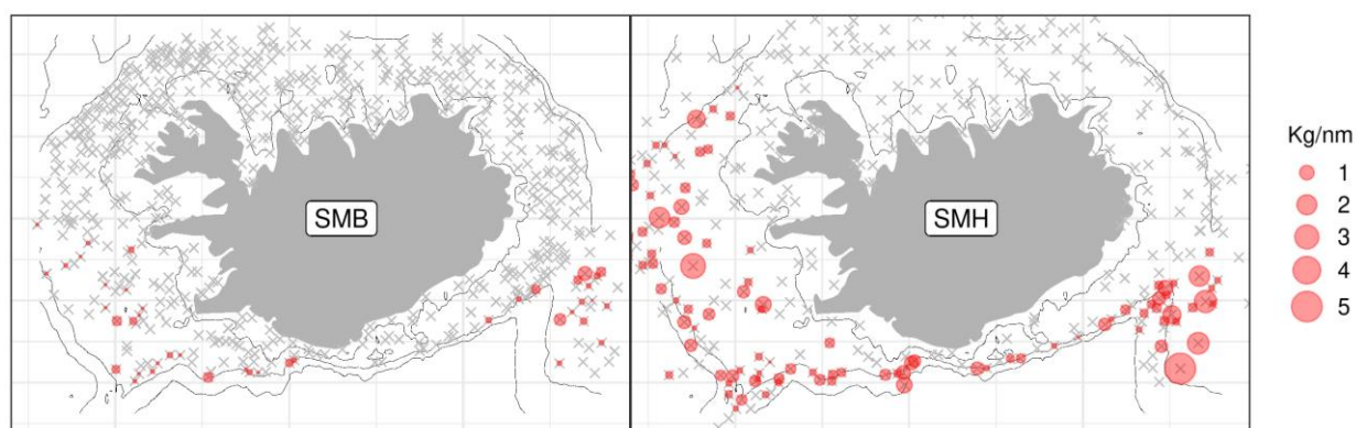
Figure 9. Blue ling. Abundance and location of blue ling in spring survey (SMB) in 2022 and autumn survey (SMH) in 2021.
