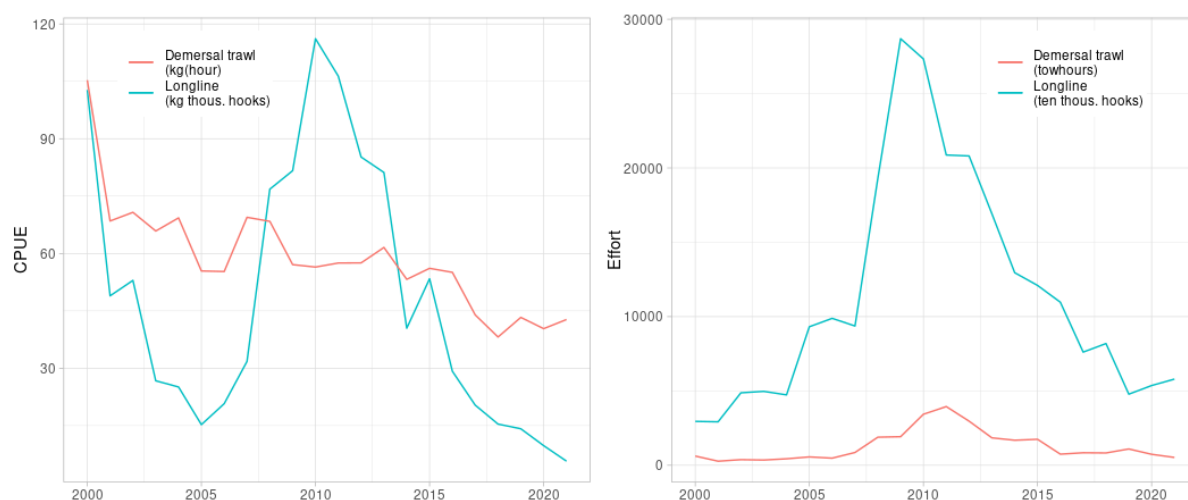
Figure 5. Blue ling. Estimates of CPUE (left) and fishing effort (right) from longlines and trawls based on logbook data where blue ling was recorded in catches.
