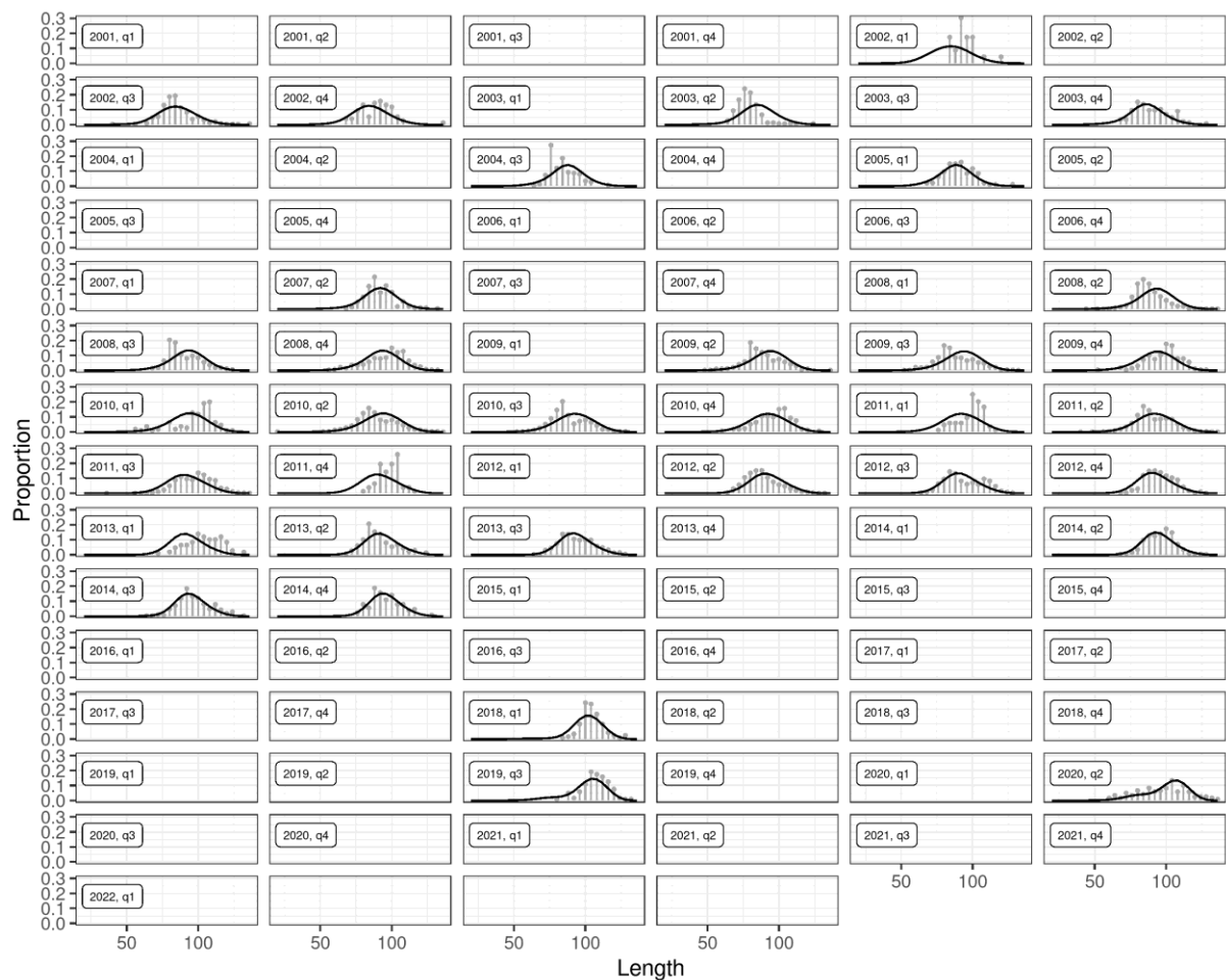
Figure 20. Blue ling. Fitted proportions-at-length from the Gadget model (black lines) compared to observed proportions from commercial catches (longline fleet).
