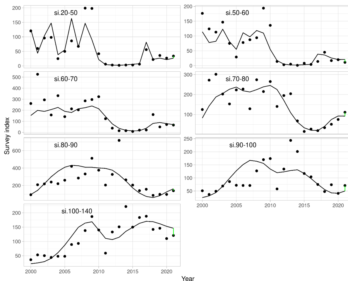
Figure 22. Blue ling. Fitted autumn survey index by length group from the Gadget model (black line) and the observed number of blue ling caught in the survey (points). The green line indicates the difference between the terminal fit and the observations.
