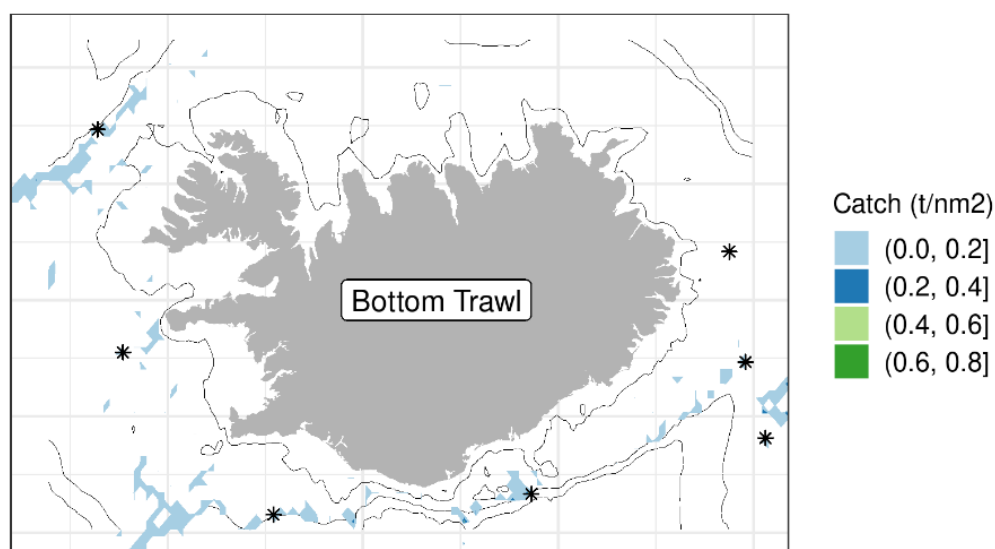
Figure 6. Blue ling. Spatial distribution of length samples (black dots) from commercial catches in Icelandic waters in 2021.
