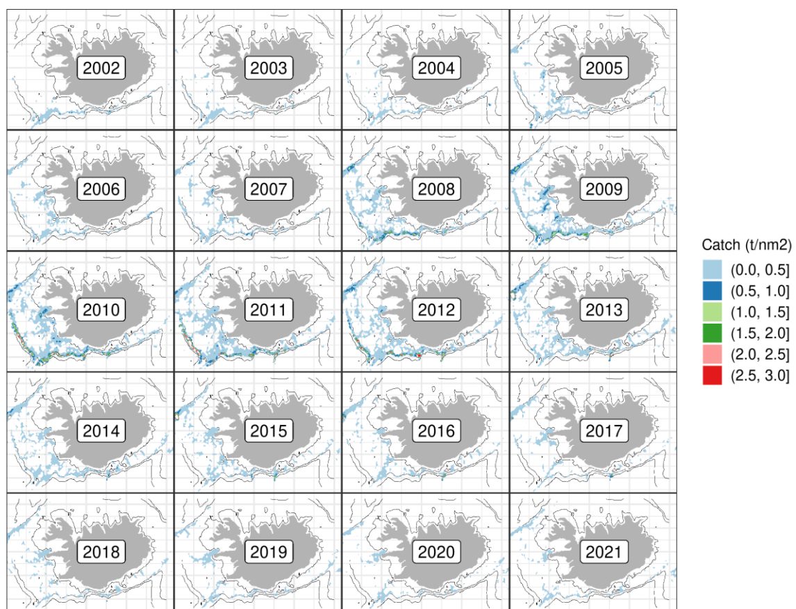
Figure 1. Blue ling. Geographic distribution of the Icelandic fishery since 2002 as reported in logbooks.
